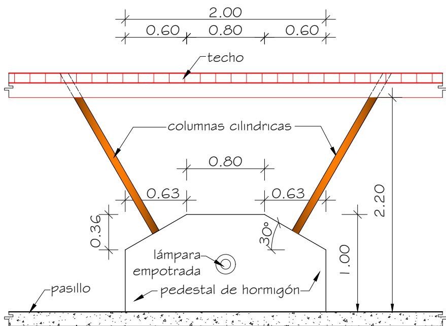
DETALLE DE COBERTIZO-PATIO INTERIOR
